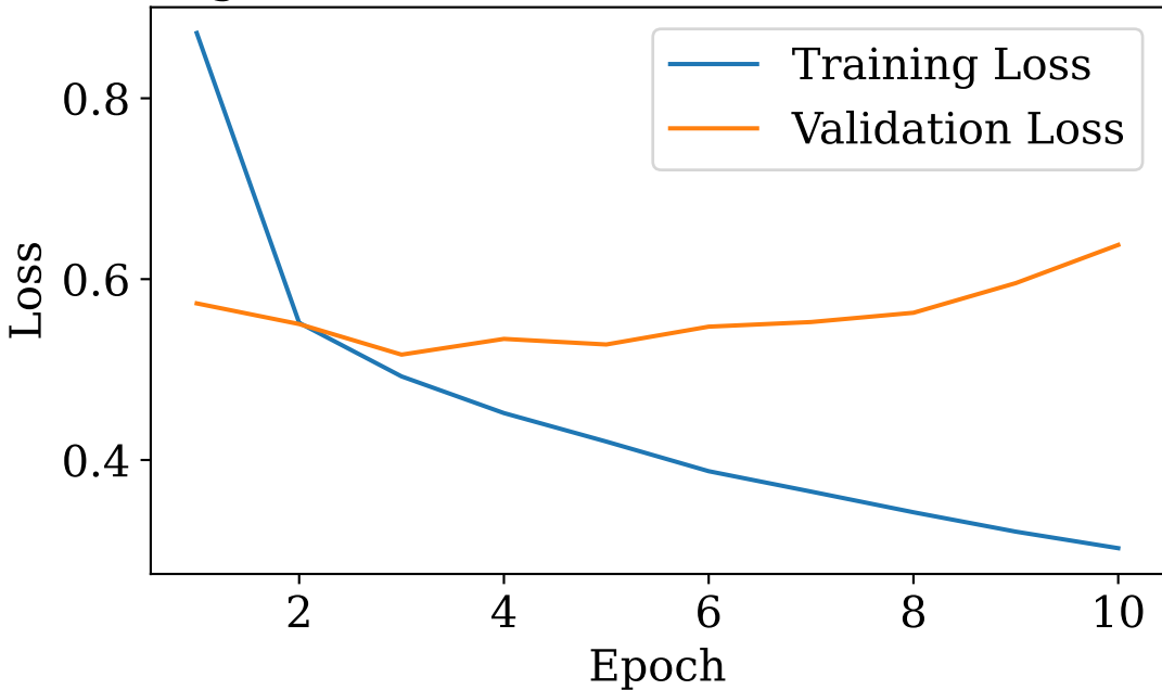
Training vs Validation Loss (Before Fine-Tuning)
